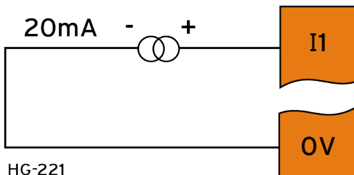
20mA Analog In - Self-Powered
