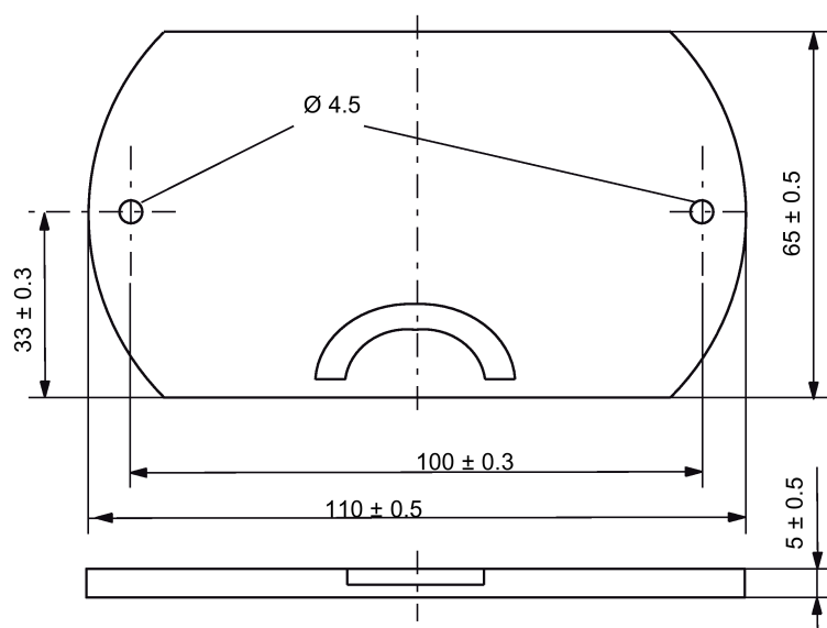
Figure A-8 Dimension drawing of fixing pocket 6GT2390-0AA00
