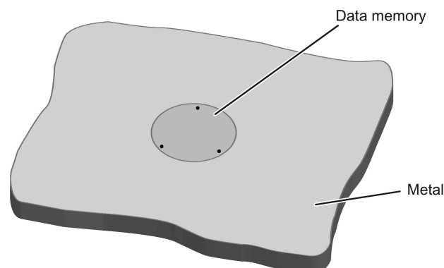
Figure 7-40 Mounting of MDS D422 in metal
