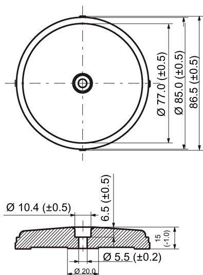
Figure 7-30 Dimension drawing of the MDS D339
