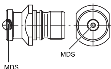
Figure 7-38 Installation example of MDS D421 in a stud bolt
