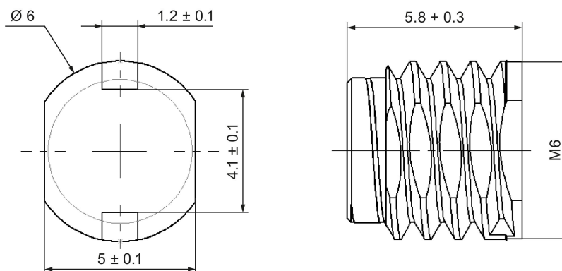
Figure 7-11 Dimensions in mm
