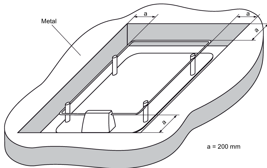
Figure 6-31 Metal-free area for ANT D6
