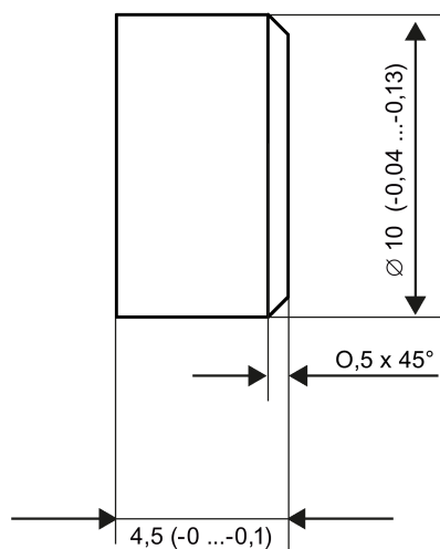
Figure 7-39 Dimension drawing of MDS D421
