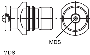
Figure 7-61 Installation example of MDS D521 in a stud bolt
