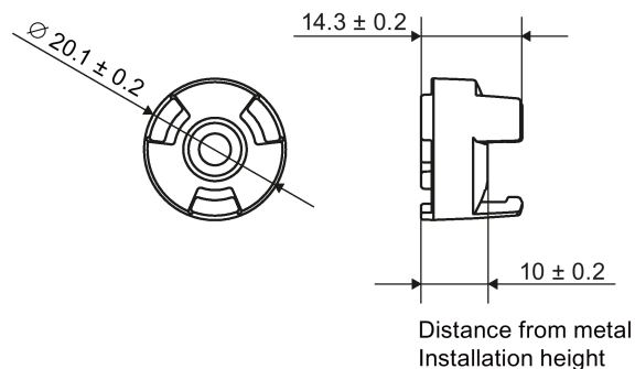
Figure 7-56 Dimensional drawing of spacer
