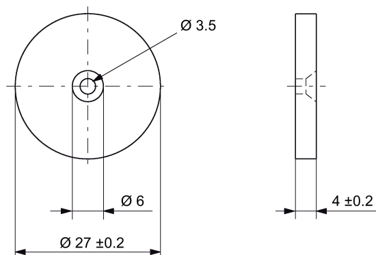
Figure 7-8 Dimension drawing of MDS D124
