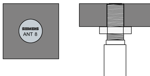
Figure 6-7 ANT 8 flush-mounted in metal
