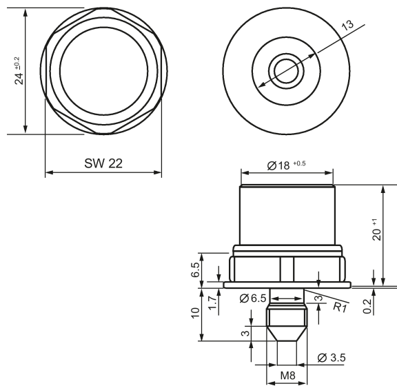
Dimensions in mm Figure 7-53 Dimension drawing of MDS D428
