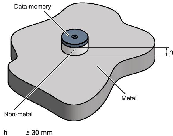
Figure 7-27 Mounting the MDS D339 on metal with spacer
