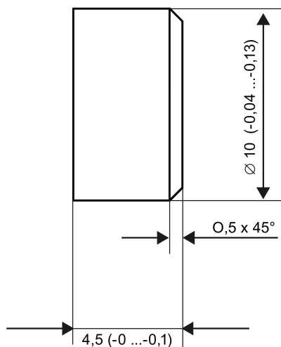
Figure 7-62 Dimensional drawing of MDS D521
