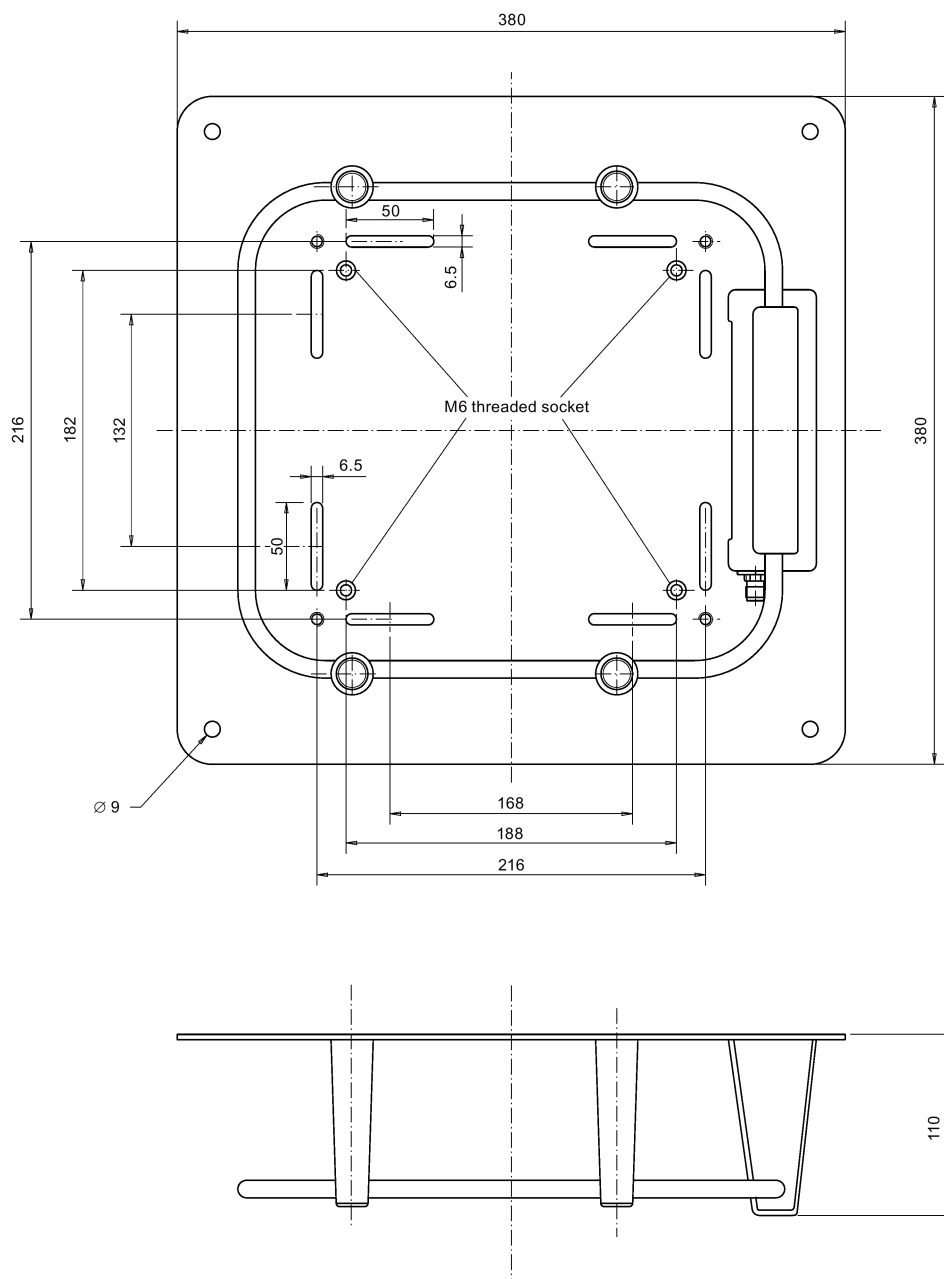
Figure 6-29 Dimension drawing for ANT D5
