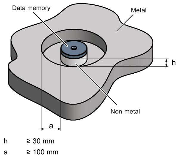
Figure 7-28 Flush-mounting of the MDS D339 in metal with spacer
