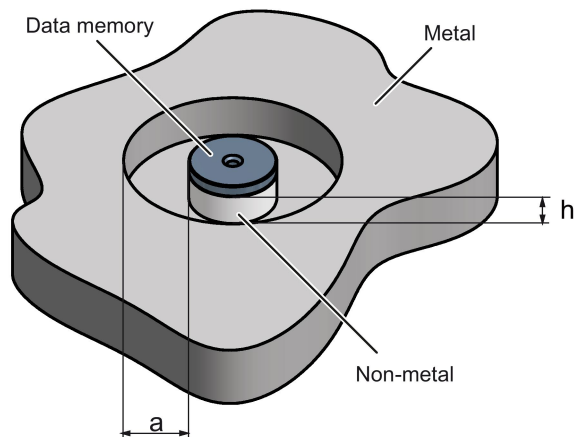
Figure 7-24 Mounting the MDS D324 on metal with spacer
