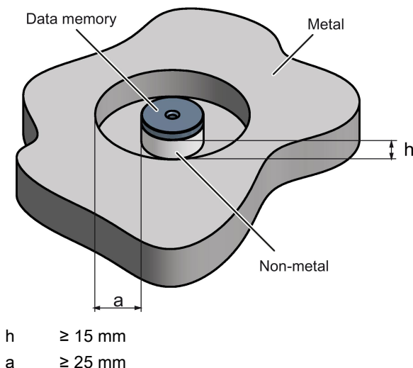
Figure 7-47 Flush-mounting of the MDS D424 in metal with spacer
