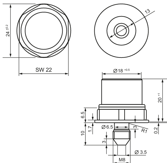
Figure 7-73 Dimensional drawing of MDS D528
