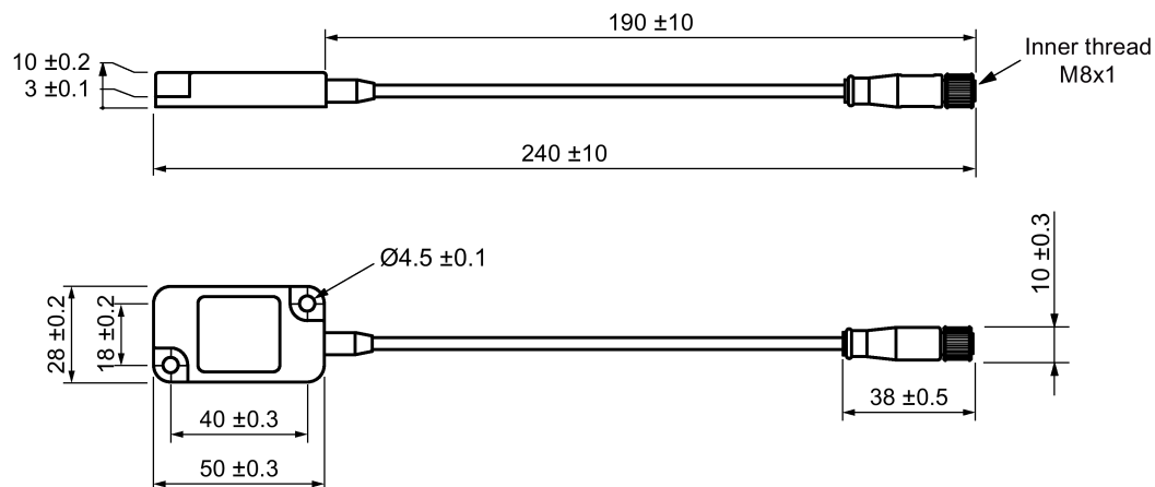
Figure 6-5 Dimension drawing ANT 3 (all values in mm)
