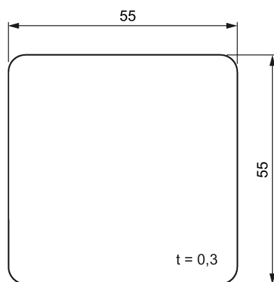
Figure 7-23 Dimension drawing of MDS D261
